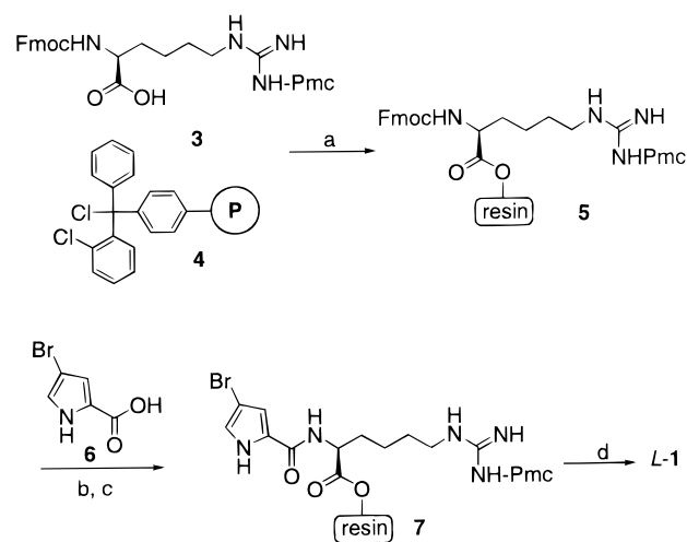
Scheme 1. Solid-Phase Synthesis of L- 1 a
